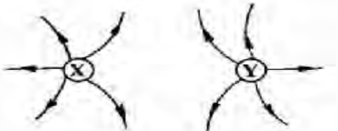
The electric field between the two-point charges
